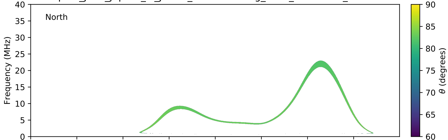
expres_juno_jupiter_io_jrm09_lossc-wid1deg_3kev_20210111_v11.cdf
