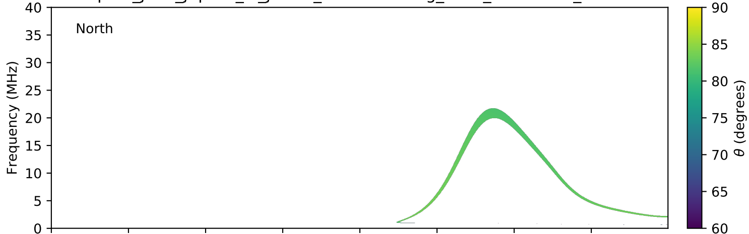
expres_juno_jupiter_io_jrm09_lossc-wid1deg_3kev_20210109_v11.cdf
