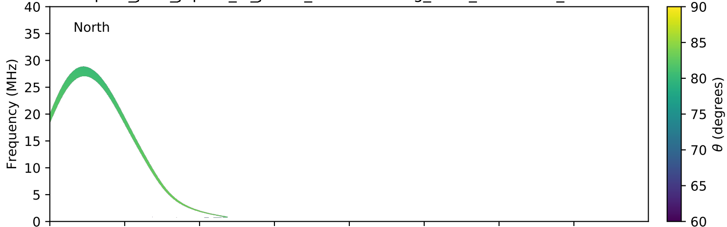
expres_juno_jupiter_io_jrm09_lossc-wid1deg_3kev_20210108_v11.cdf
