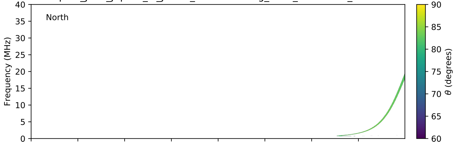
expres_juno_jupiter_io_jrm09_lossc-wid1deg_3kev_20210107_v11.cdf
