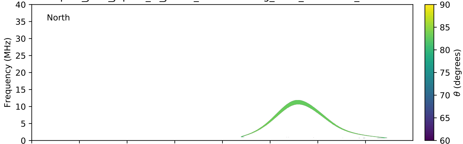
expres_juno_jupiter_io_jrm09_lossc-wid1deg_3kev_20210102_v11.cdf
