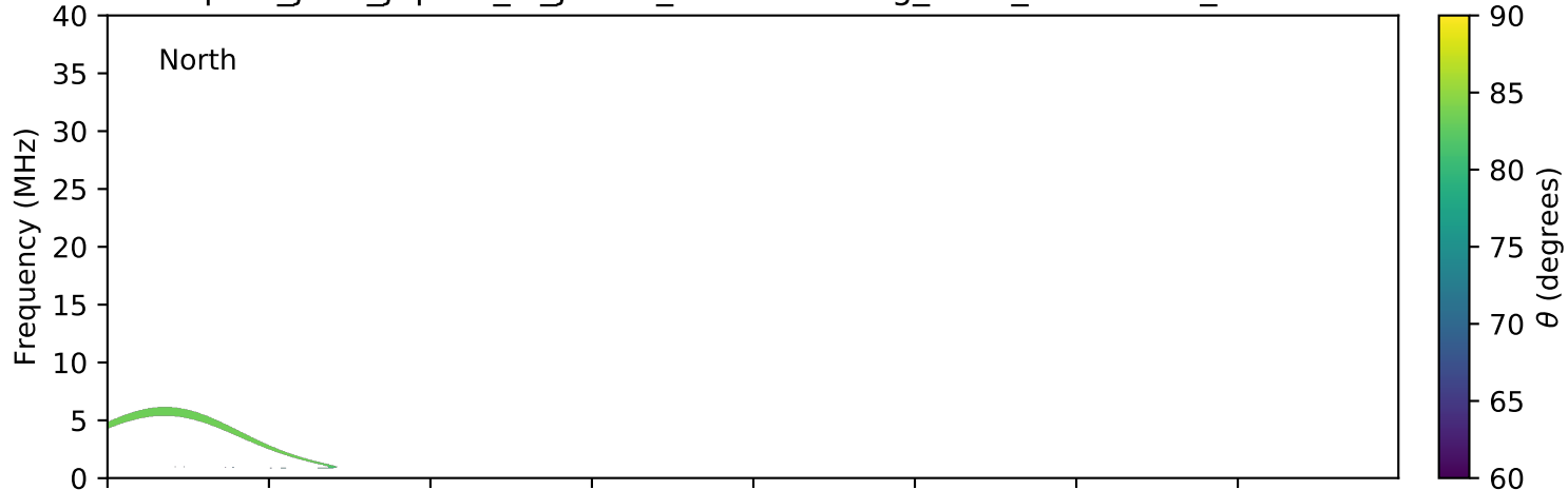
expres_juno_jupiter_io_jrm09_lossc-wid1deg_3kev_20210101_v11.cdf
