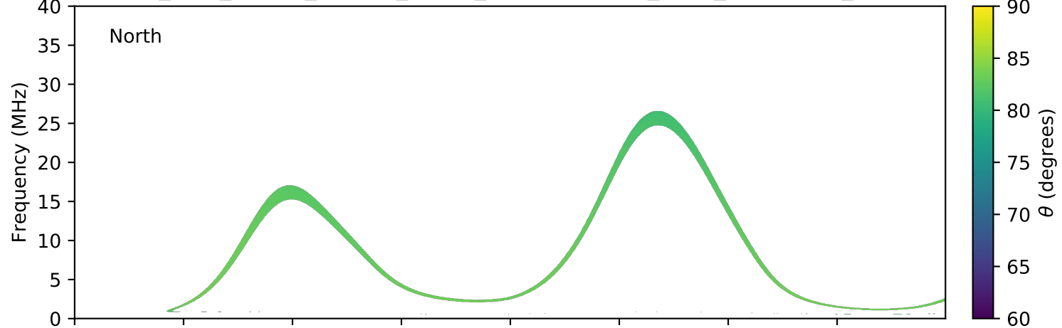
expres_juno_jupiter_europa_jrm09_lossc-wid1deg_3kev_20210126_v11.cdf
