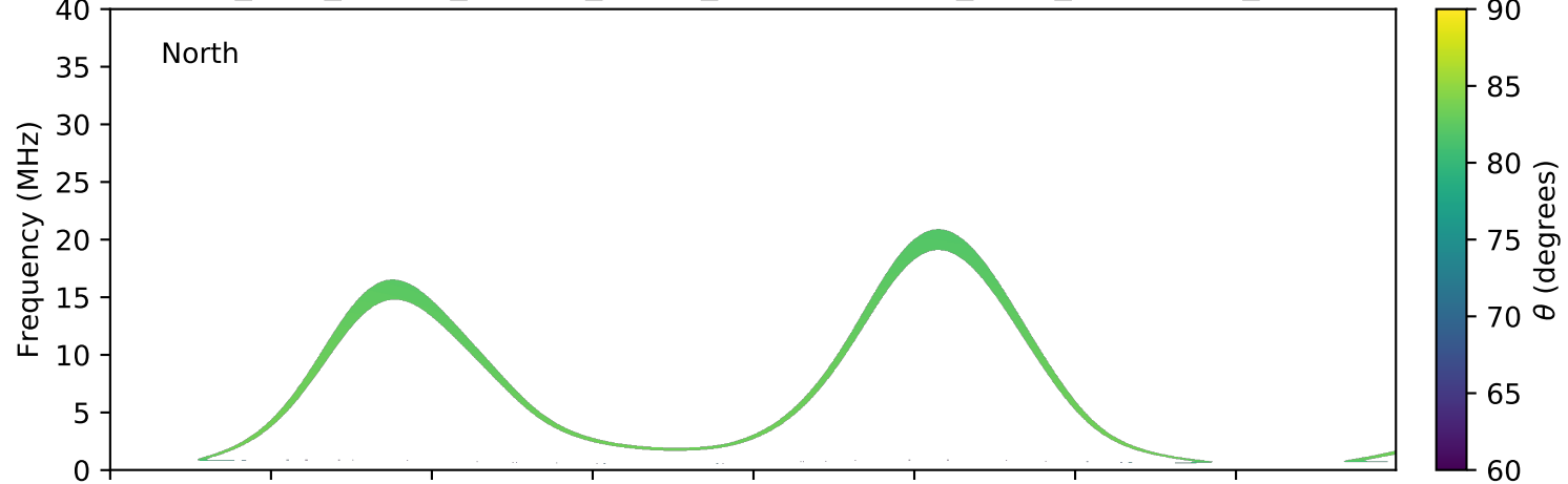
expres_juno_jupiter_europa_jrm09_lossc-wid1deg_3kev_20210119_v11.cdf
