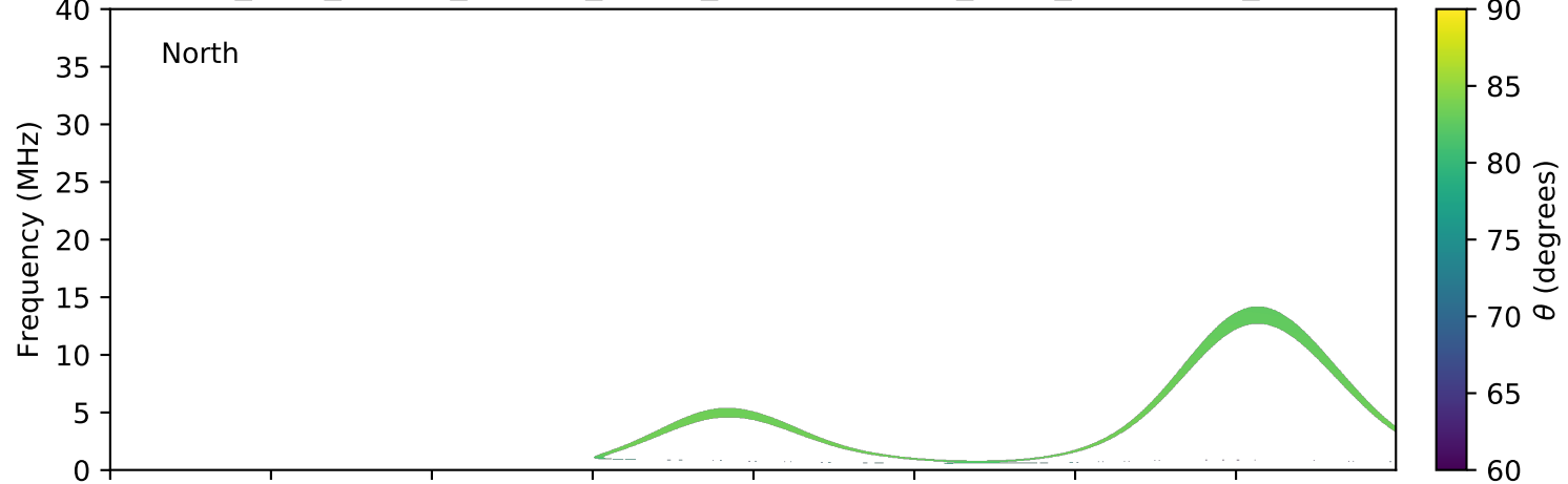
expres_juno_jupiter_europa_jrm09_lossc-wid1deg_3kev_20210108_v11.cdf
