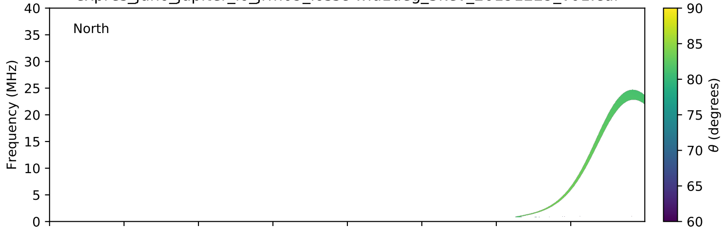
expres_juno_jupiter_io_jrm09_lossc-wid1deg_3kev_20191229_v01.cdf
