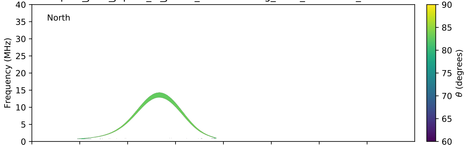
expres_juno_jupiter_io_jrm09_lossc-wid1deg_3kev_20191228_v01.cdf
