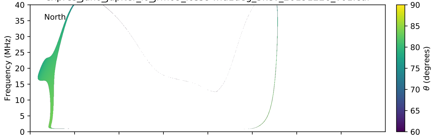
expres_juno_jupiter_io_jrm09_lossc-wid1deg_3kev_20191226_v01.cdf
