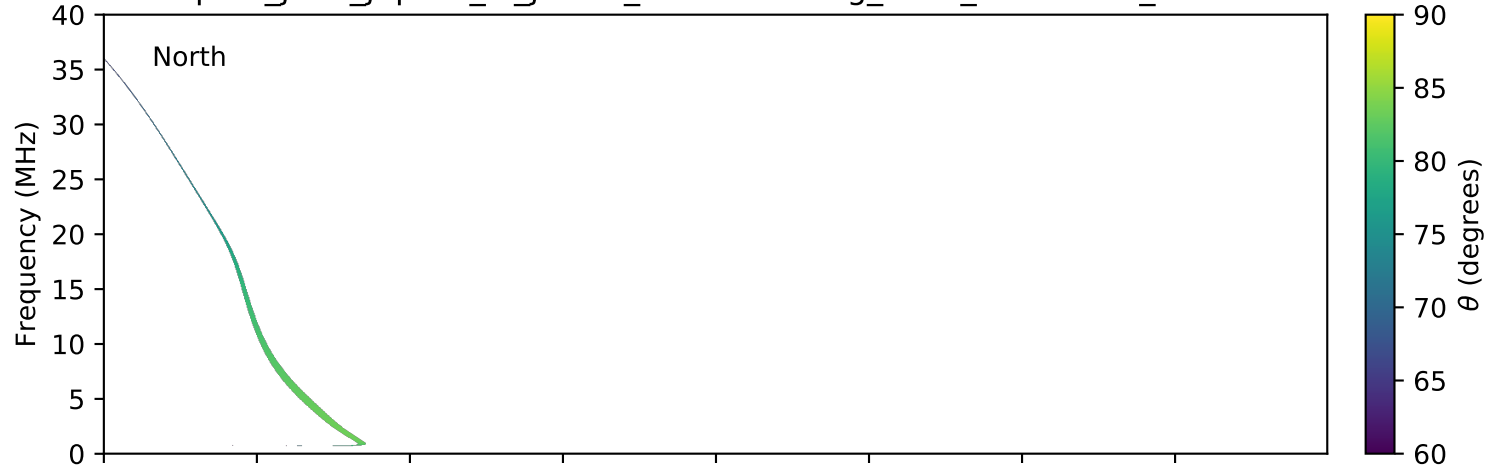
expres_juno_jupiter_io_jrm09_lossc-wid1deg_3kev_20191223_v01.cdf
