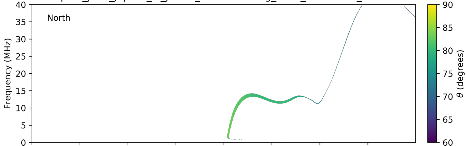
expres_juno_jupiter_io_jrm09_lossc-wid1deg_3kev_20191222_v01.cdf
