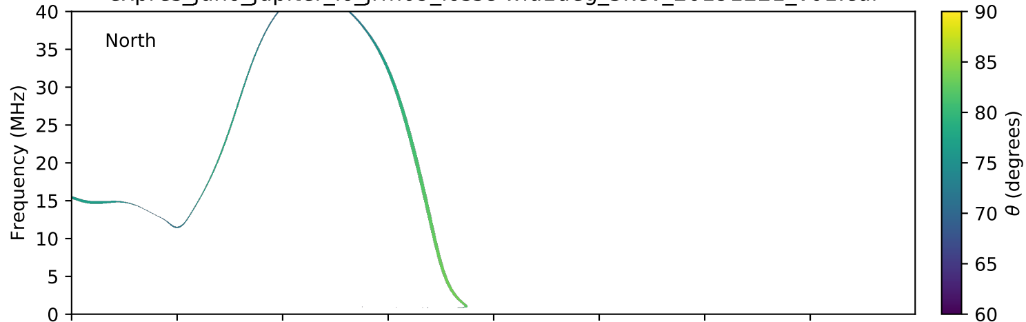
expres_juno_jupiter_io_jrm09_lossc-wid1deg_3kev_20191221_v01.cdf
