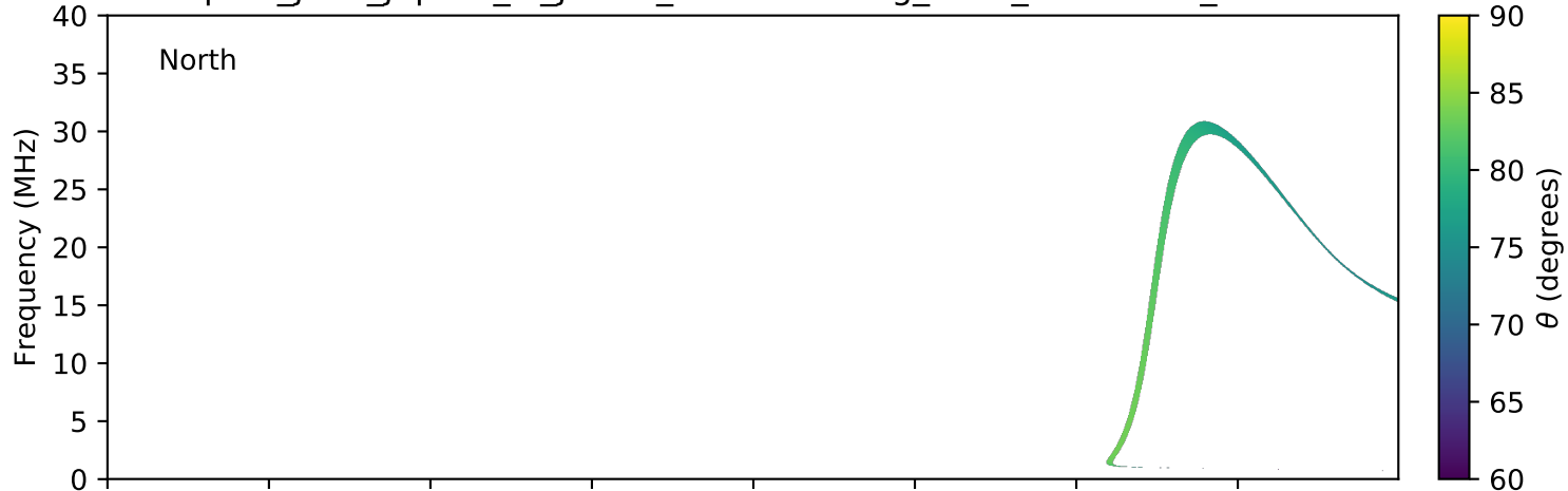
expres_juno_jupiter_io_jrm09_lossc-wid1deg_3kev_20191220_v01.cdf
