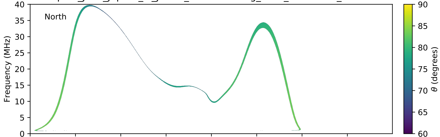
expres_juno_jupiter_io_jrm09_lossc-wid1deg_3kev_20191219_v01.cdf
