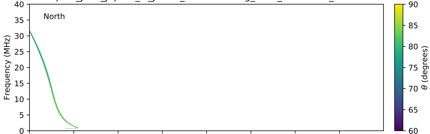
expres_juno_jupiter_io_jrm09_lossc-wid1deg_3kev_20191216_v01.cdf
