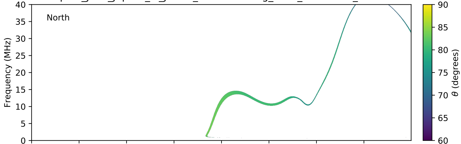
expres_juno_jupiter_io_jrm09_lossc-wid1deg_3kev_20191215_v01.cdf
