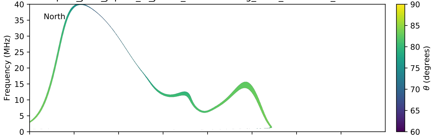
expres_juno_jupiter_io_jrm09_lossc-wid1deg_3kev_20191212_v01.cdf
