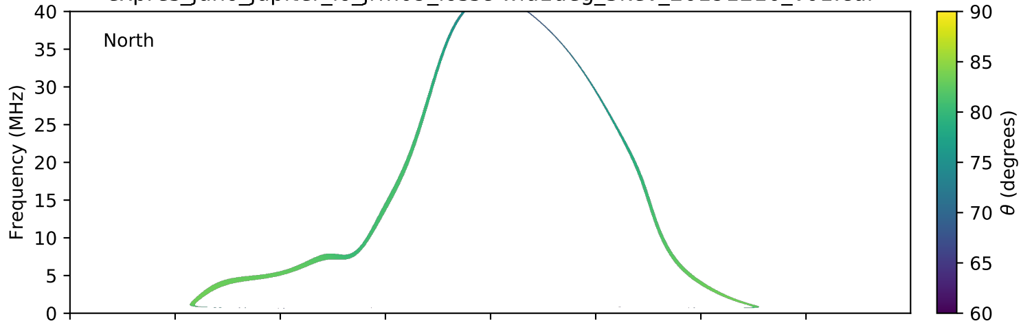
expres_juno_jupiter_io_jrm09_lossc-wid1deg_3kev_20191210_v01.cdf
