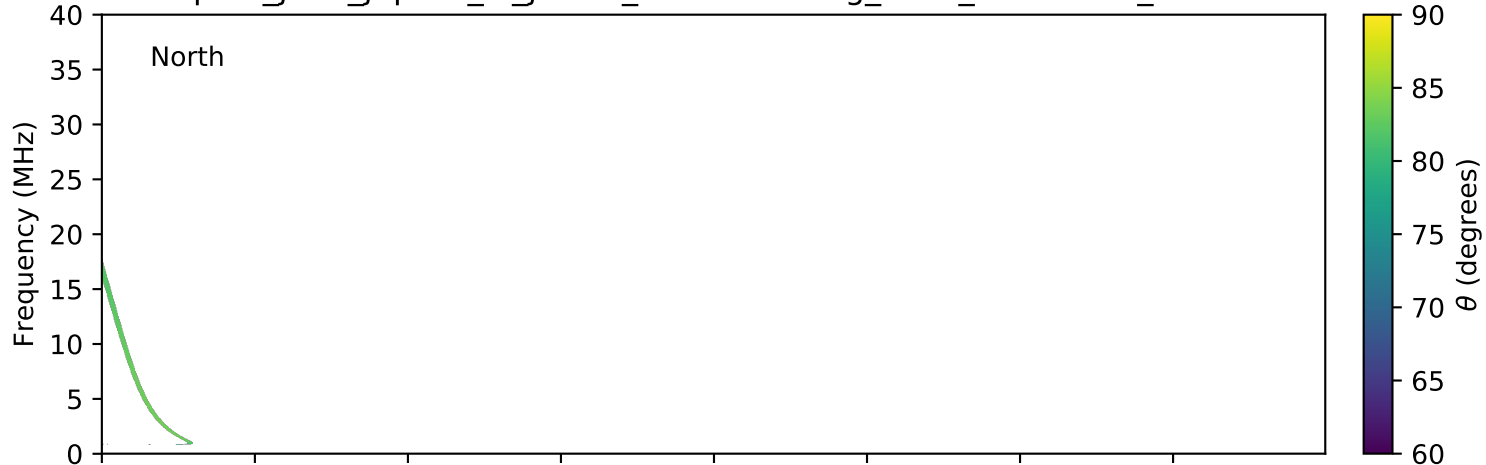
expres_juno_jupiter_io_jrm09_lossc-wid1deg_3kev_20191209_v01.cdf
