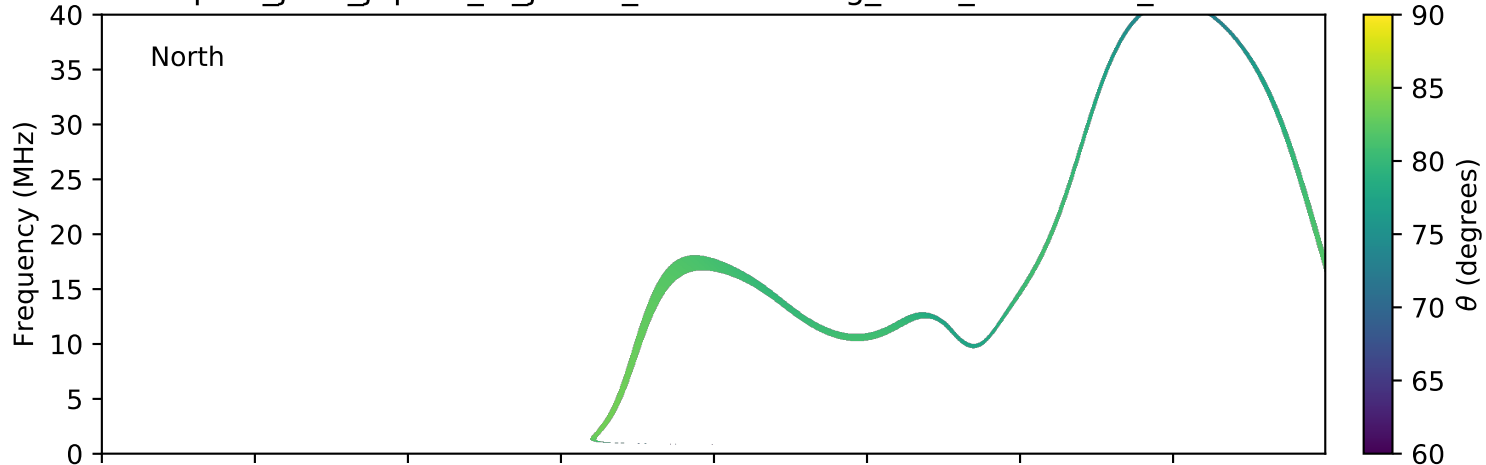
expres_juno_jupiter_io_jrm09_lossc-wid1deg_3kev_20191208_v01.cdf
