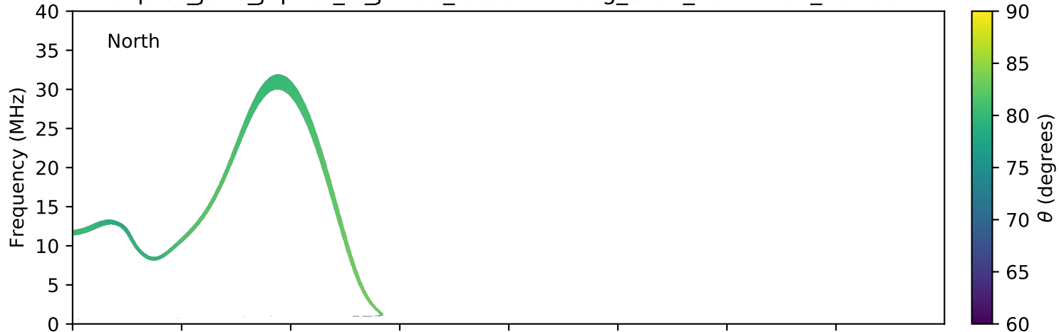
expres_juno_jupiter_io_jrm09_lossc-wid1deg_3kev_20191207_v01.cdf
