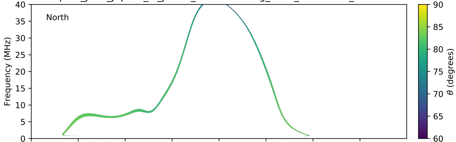
expres_juno_jupiter_io_jrm09_lossc-wid1deg_3kev_20191203_v01.cdf
