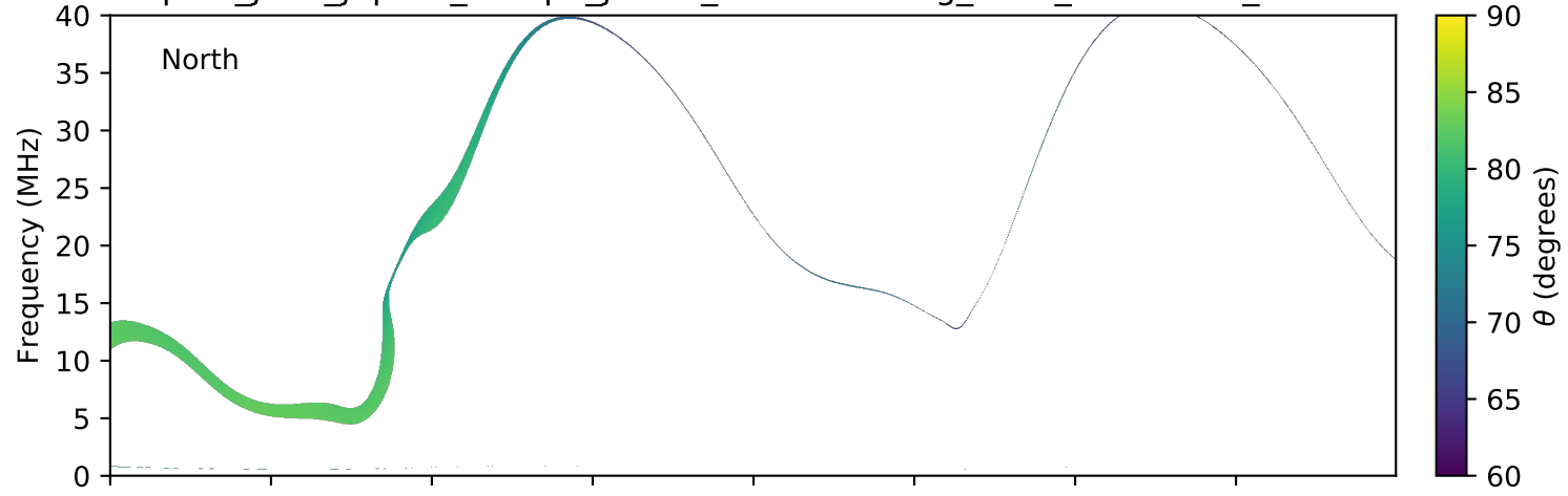
expres_juno_jupiter_europa_jrm09_lossc-wid1deg_3kev_20191225_v01.cdf
