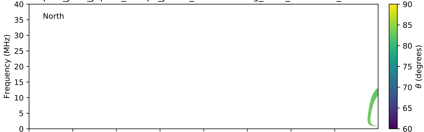
expres_juno_jupiter_europa_jrm09_lossc-wid1deg_3kev_20191224_v01.cdf
