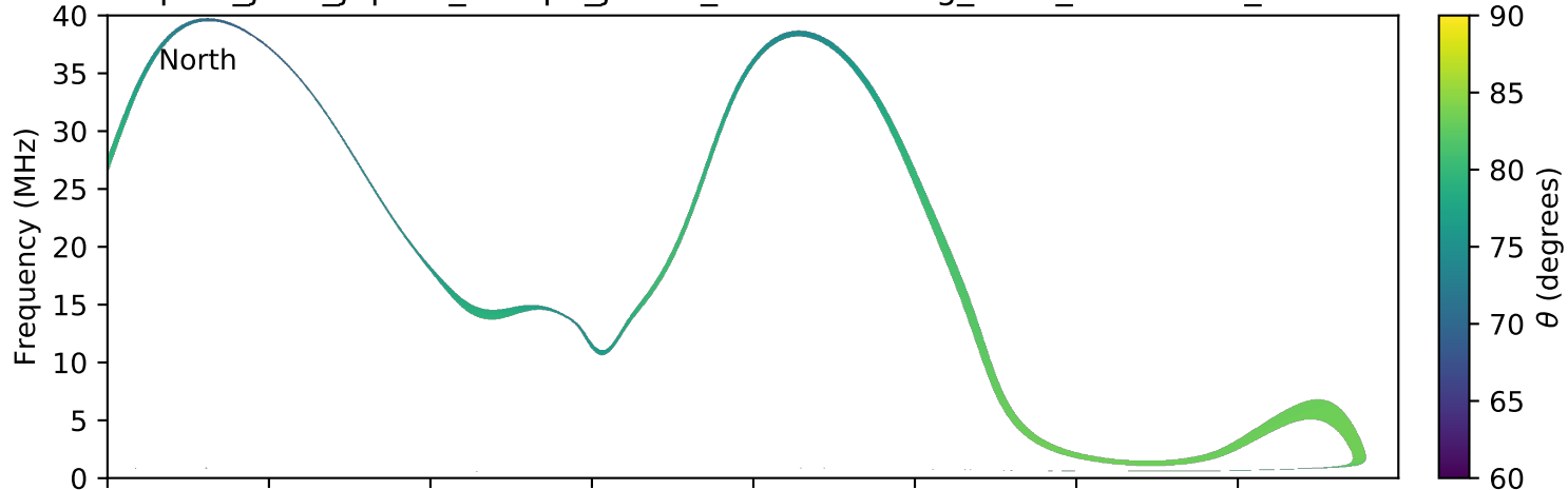
expres_juno_jupiter_europa_jrm09_lossc-wid1deg_3kev_20191222_v01.cdf
