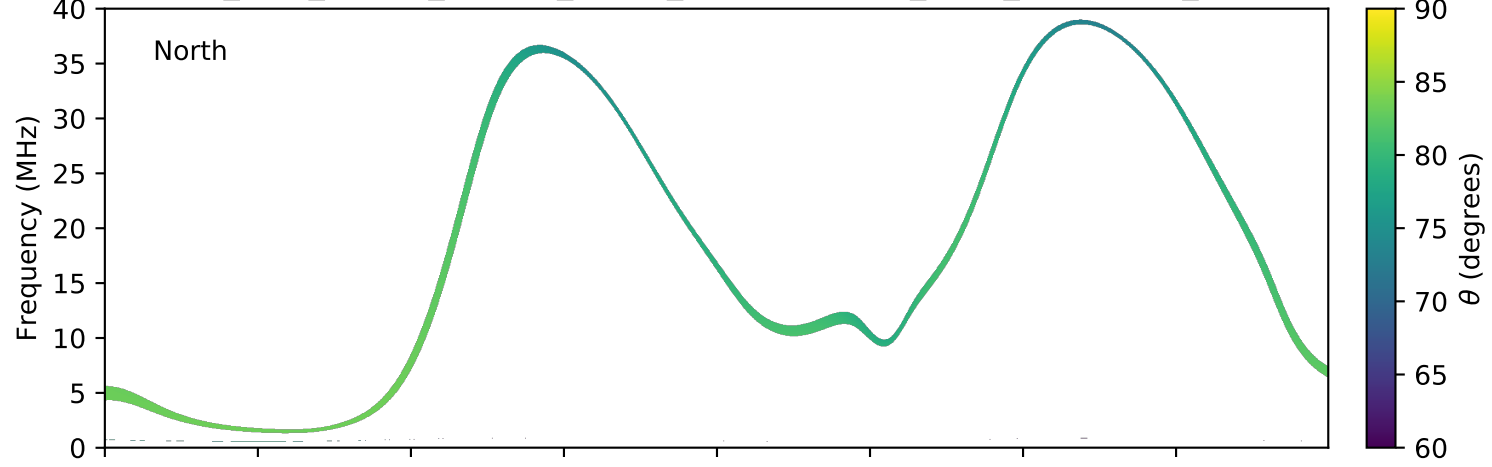
expres_juno_jupiter_europa_jrm09_lossc-wid1deg_3kev_20191218_v01.cdf
