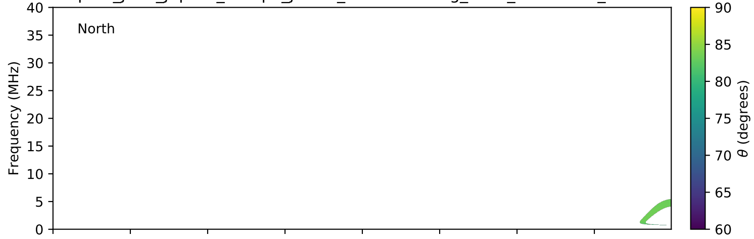
expres_juno_jupiter_europa_jrm09_lossc-wid1deg_3kev_20191217_v01.cdf
