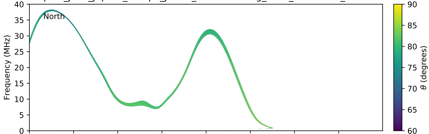
expres_juno_jupiter_europa_jrm09_lossc-wid1deg_3kev_20191215_v01.cdf
