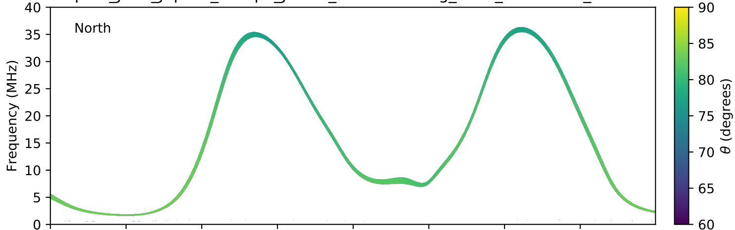
expres_juno_jupiter_europa_jrm09_lossc-wid1deg_3kev_20191211_v01.cdf
