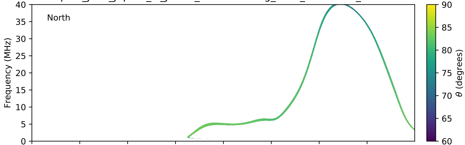
expres_juno_jupiter_io_jrm09_lossc-wid1deg_3kev_20190930_v01.cdf
