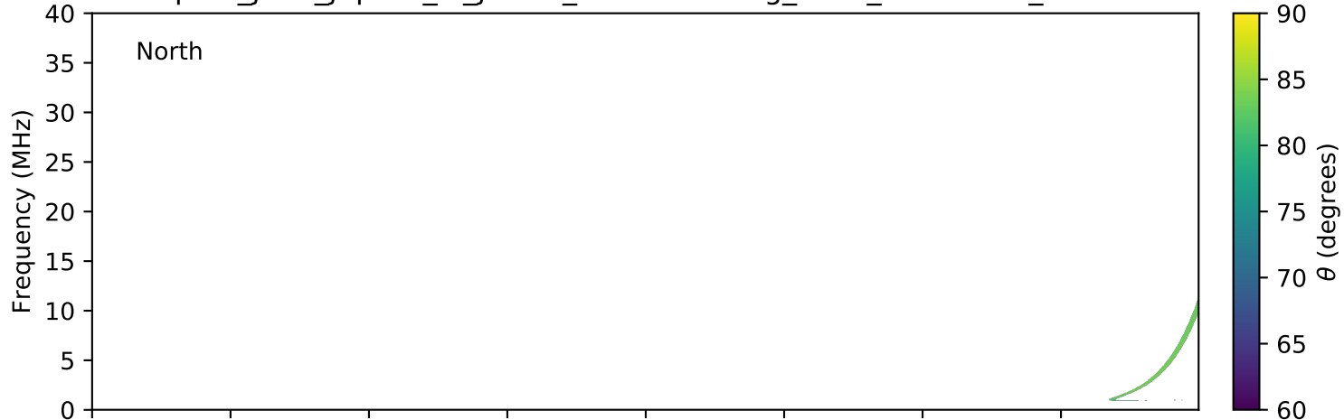
expres_juno_jupiter_io_jrm09_lossc-wid1deg_3kev_20190926_v01.cdf
