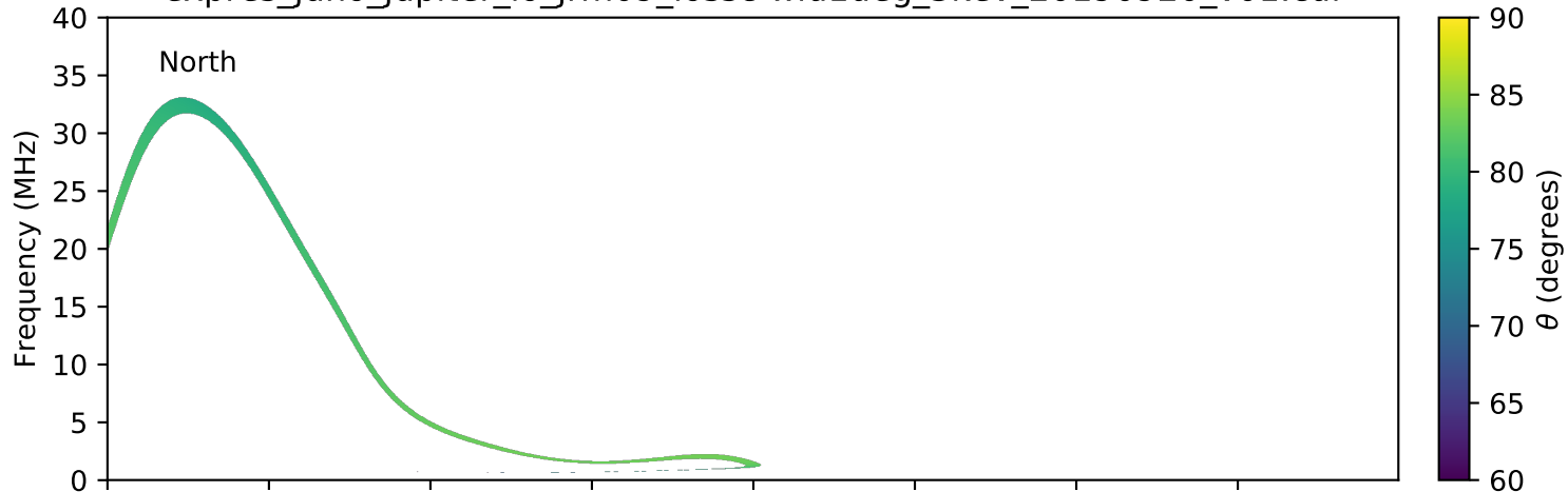
expres_juno_jupiter_io_jrm09_lossc-wid1deg_3kev_20190920_v01.cdf
