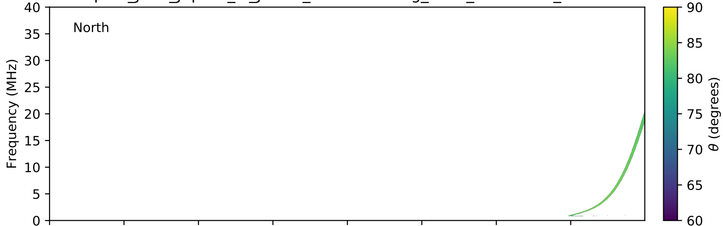
expres_juno_jupiter_io_jrm09_lossc-wid1deg_3kev_20190919_v01.cdf
