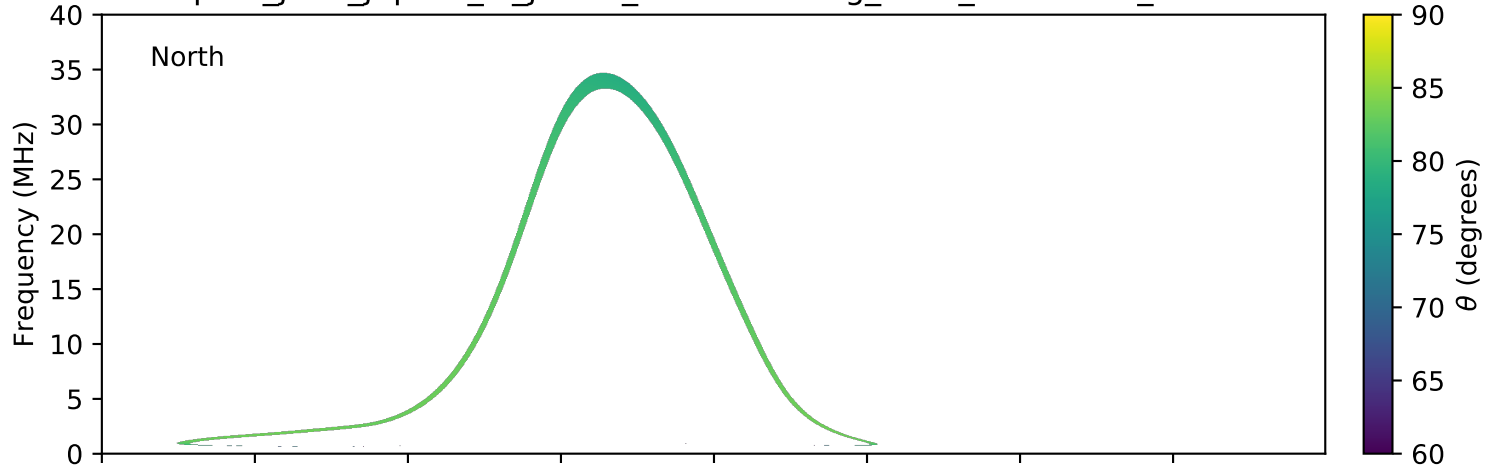
expres_juno_jupiter_io_jrm09_lossc-wid1deg_3kev_20190918_v01.cdf
