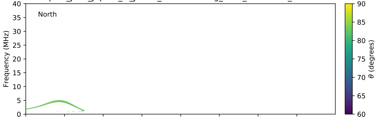
expres_juno_jupiter_io_jrm09_lossc-wid1deg_3kev_20190915_v01.cdf
