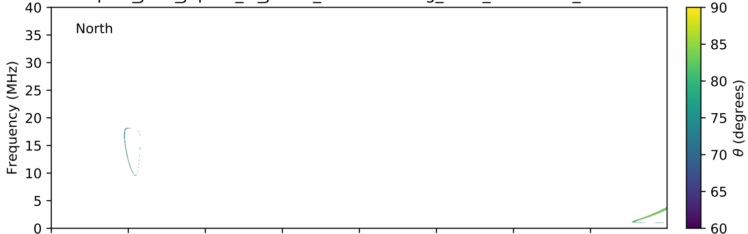
expres_juno_jupiter_io_jrm09_lossc-wid1deg_3kev_20190912_v01.cdf
