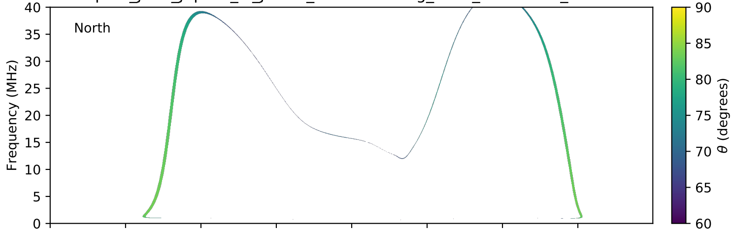
expres_juno_jupiter_io_jrm09_lossc-wid1deg_3kev_20190909_v01.cdf
