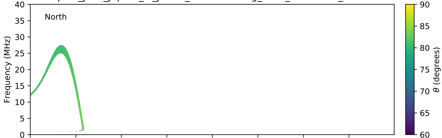
expres_juno_jupiter_io_jrm09_lossc-wid1deg_3kev_20190908_v01.cdf
