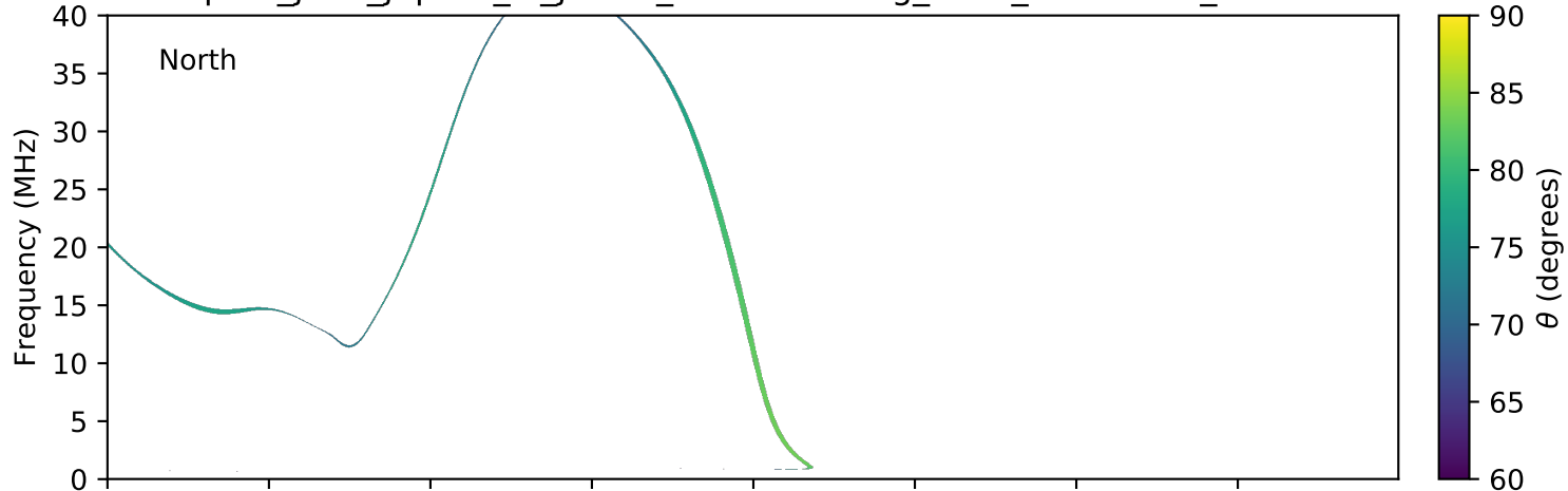
expres_juno_jupiter_io_jrm09_lossc-wid1deg_3kev_20190904_v01.cdf
