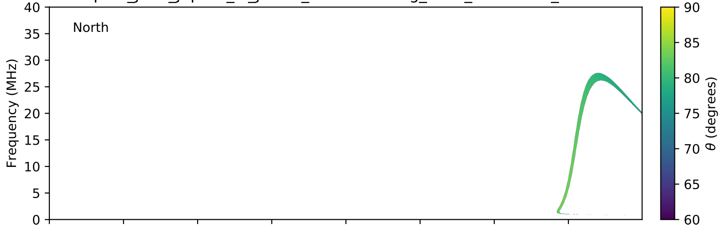
expres_juno_jupiter_io_jrm09_lossc-wid1deg_3kev_20190903_v01.cdf
