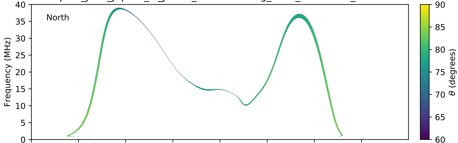
expres_juno_jupiter_io_jrm09_lossc-wid1deg_3kev_20190902_v01.cdf
