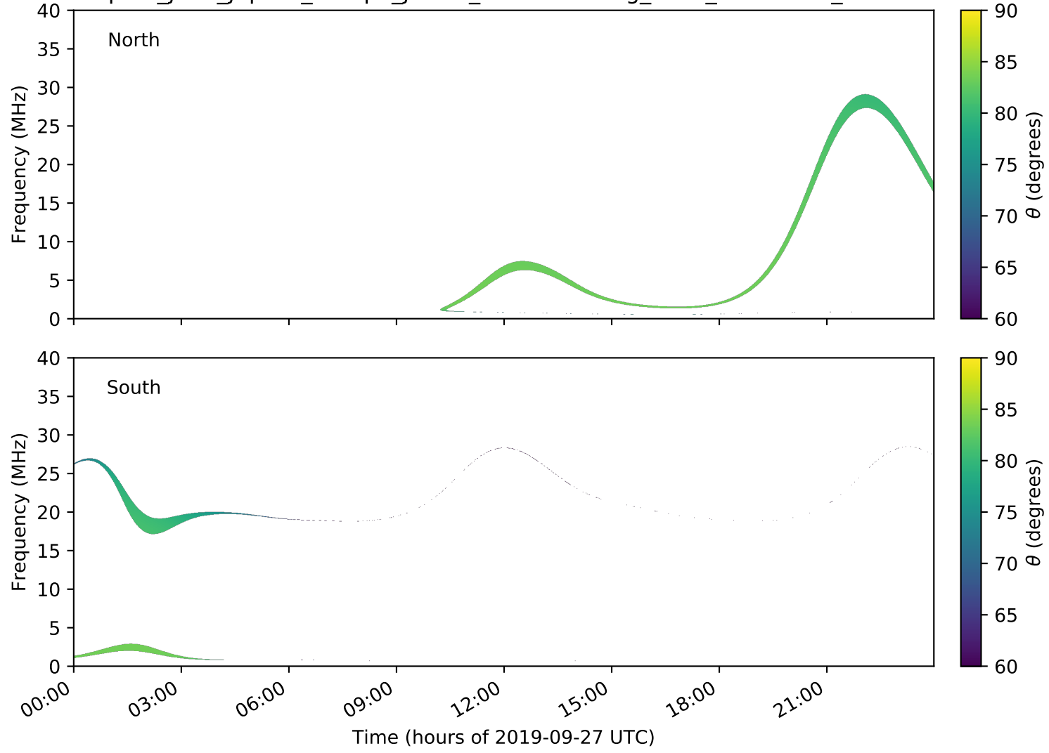
expres_juno_jupiter_europa_jrm09_lossc-wid1deg_3kev_20190927_v01.cdf
