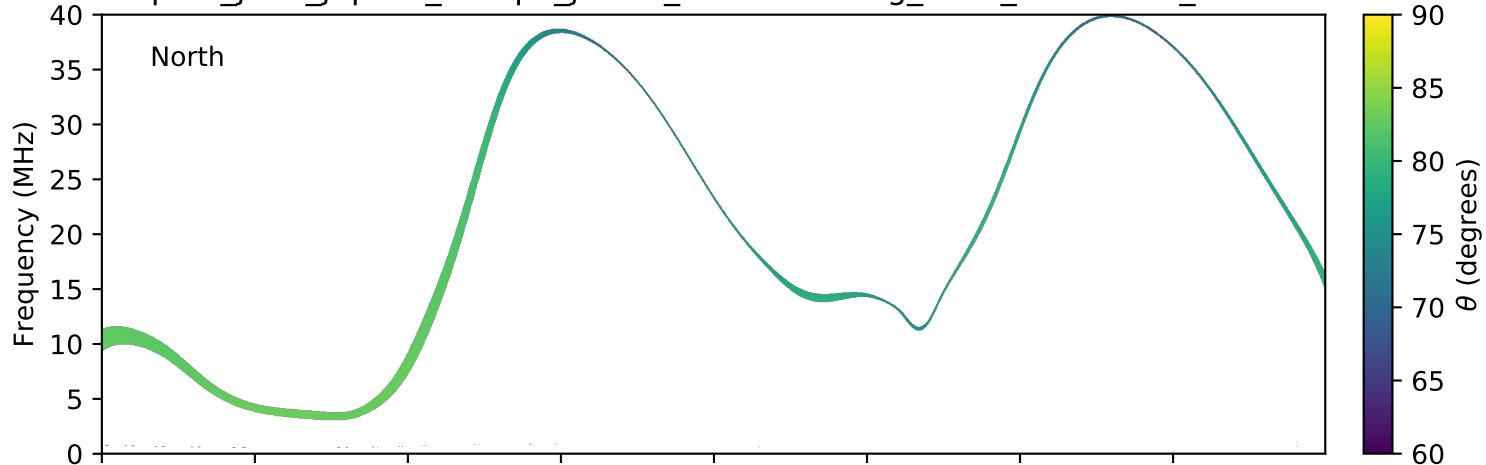
expres_juno_jupiter_europa_jrm09_lossc-wid1deg_3kev_20190906_v01.cdf
