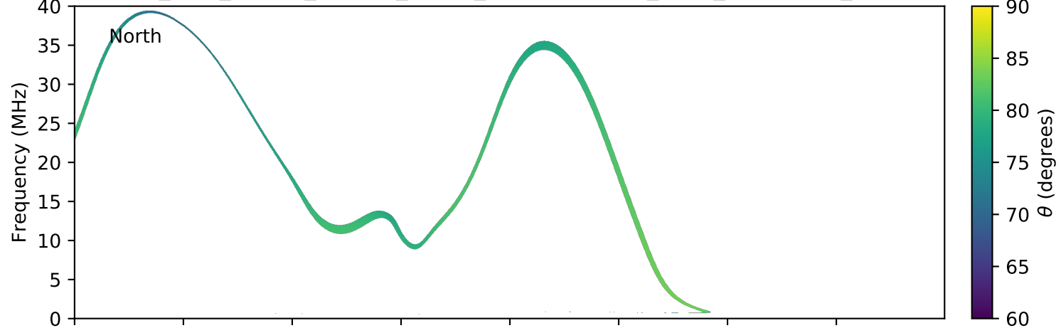
expres_juno_jupiter_europa_jrm09_lossc-wid1deg_3kev_20190903_v01.cdf
