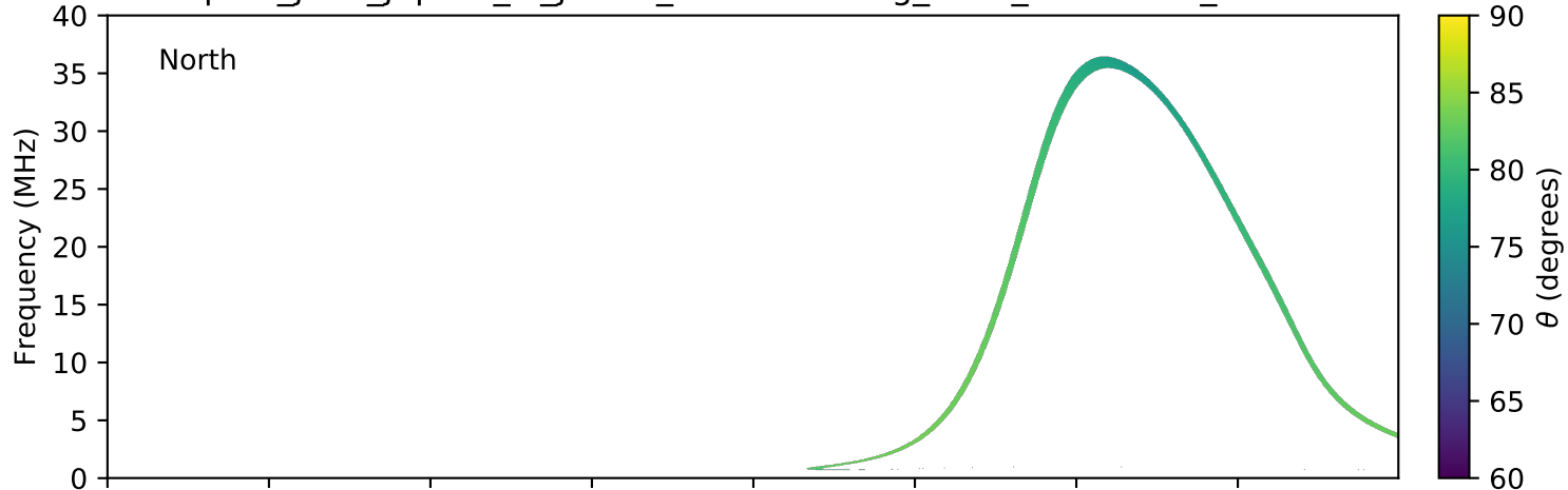
expres_juno_jupiter_io_jrm09_lossc-wid1deg_3kev_20190730_v01.cdf
