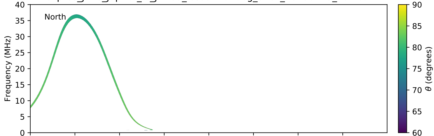
expres_juno_jupiter_io_jrm09_lossc-wid1deg_3kev_20190729_v01.cdf
