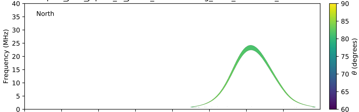
expres_juno_jupiter_io_jrm09_lossc-wid1deg_3kev_20190723_v01.cdf
